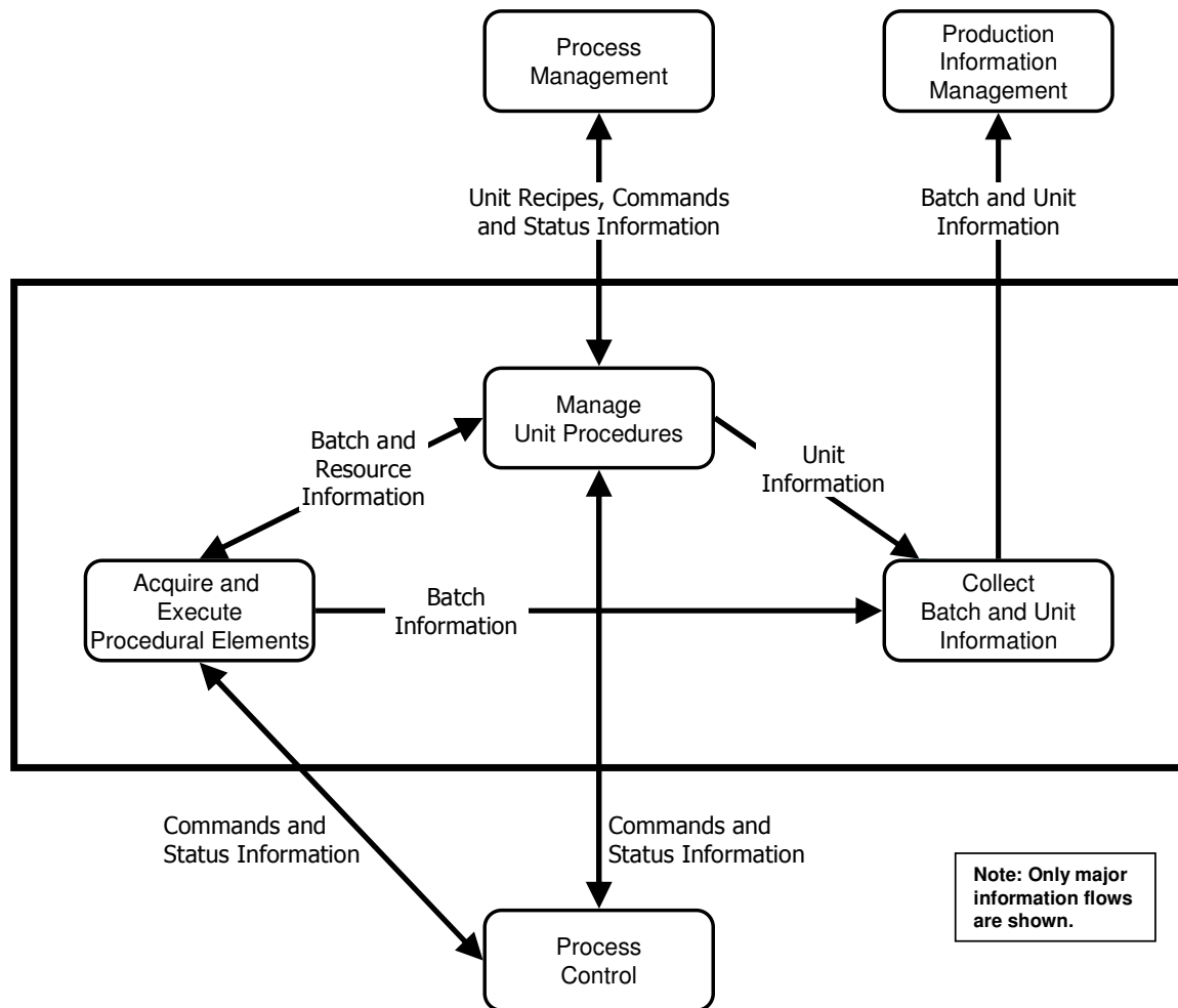
Figure 28 — Unit supervision
