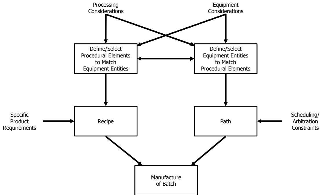
Figure 25 — Simultaneous definition/selection of procedural elements and equipment entities
