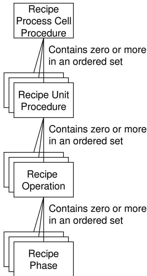
Figure 12 — Master recipe procedure levels
