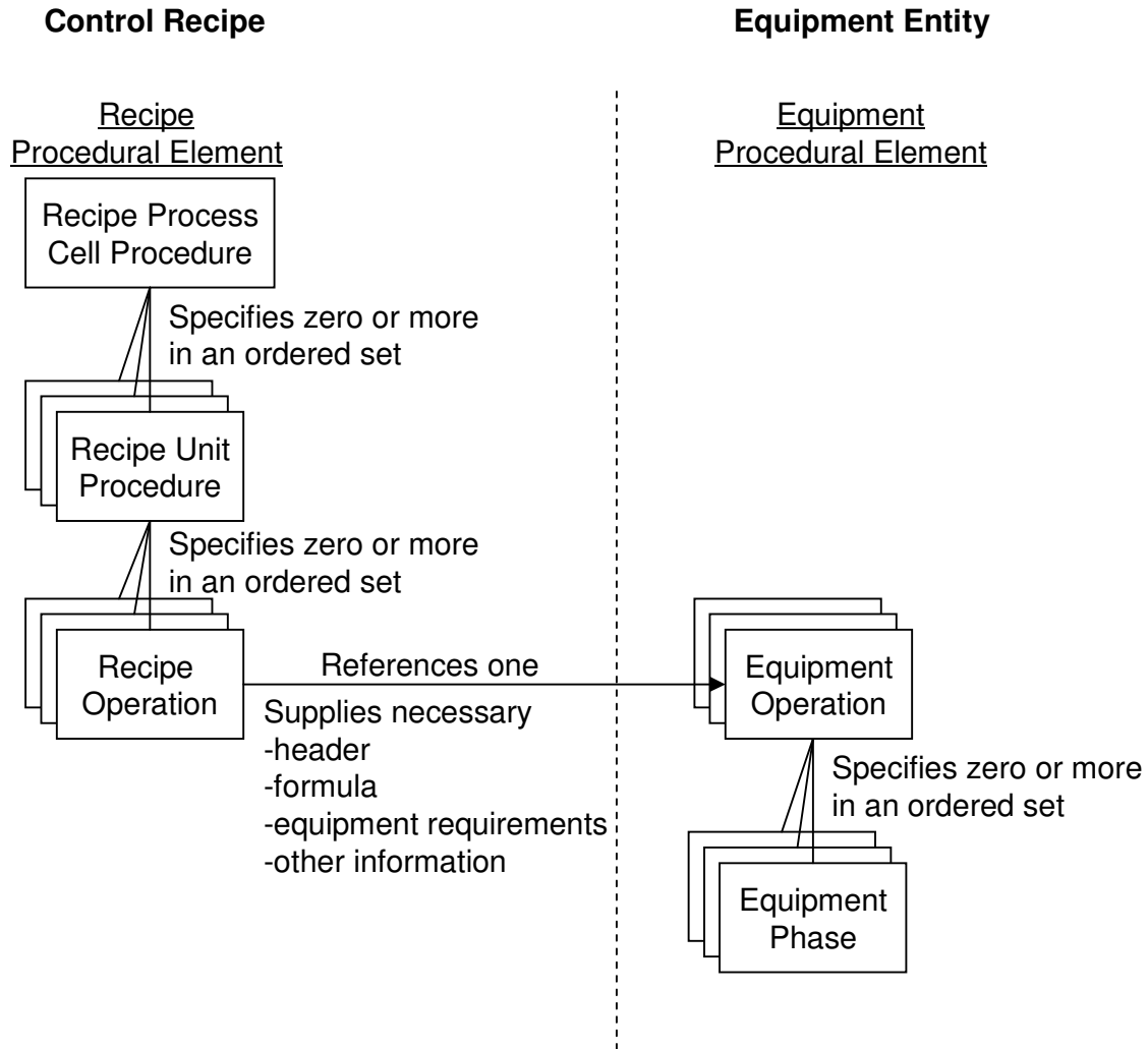
Figure 19 — Control recipe procedure example with unit procedures and operations
