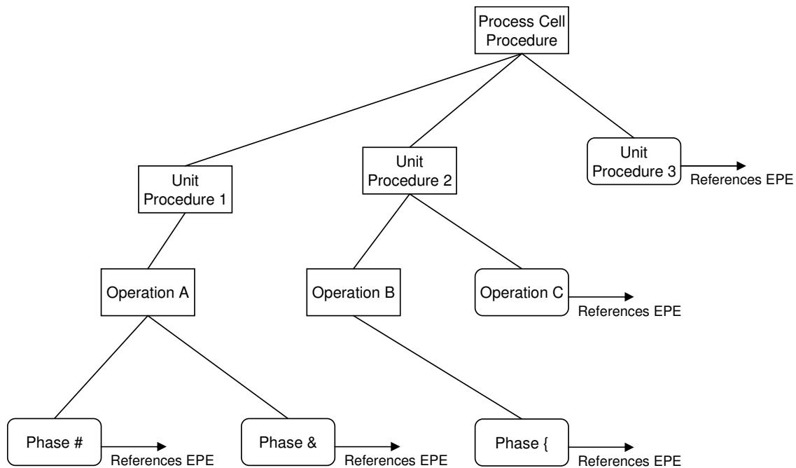
Figure 18 – Referencing equipment entities at different levels within a control recipe process cell procedure
