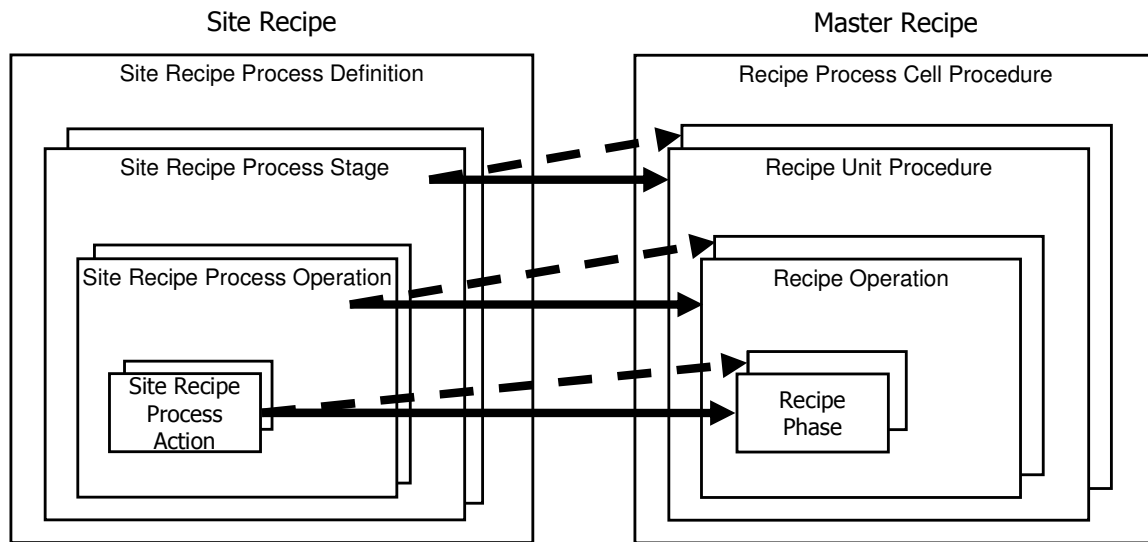
Figure 13 — Procedural element relationships in the site recipe and master recipe
