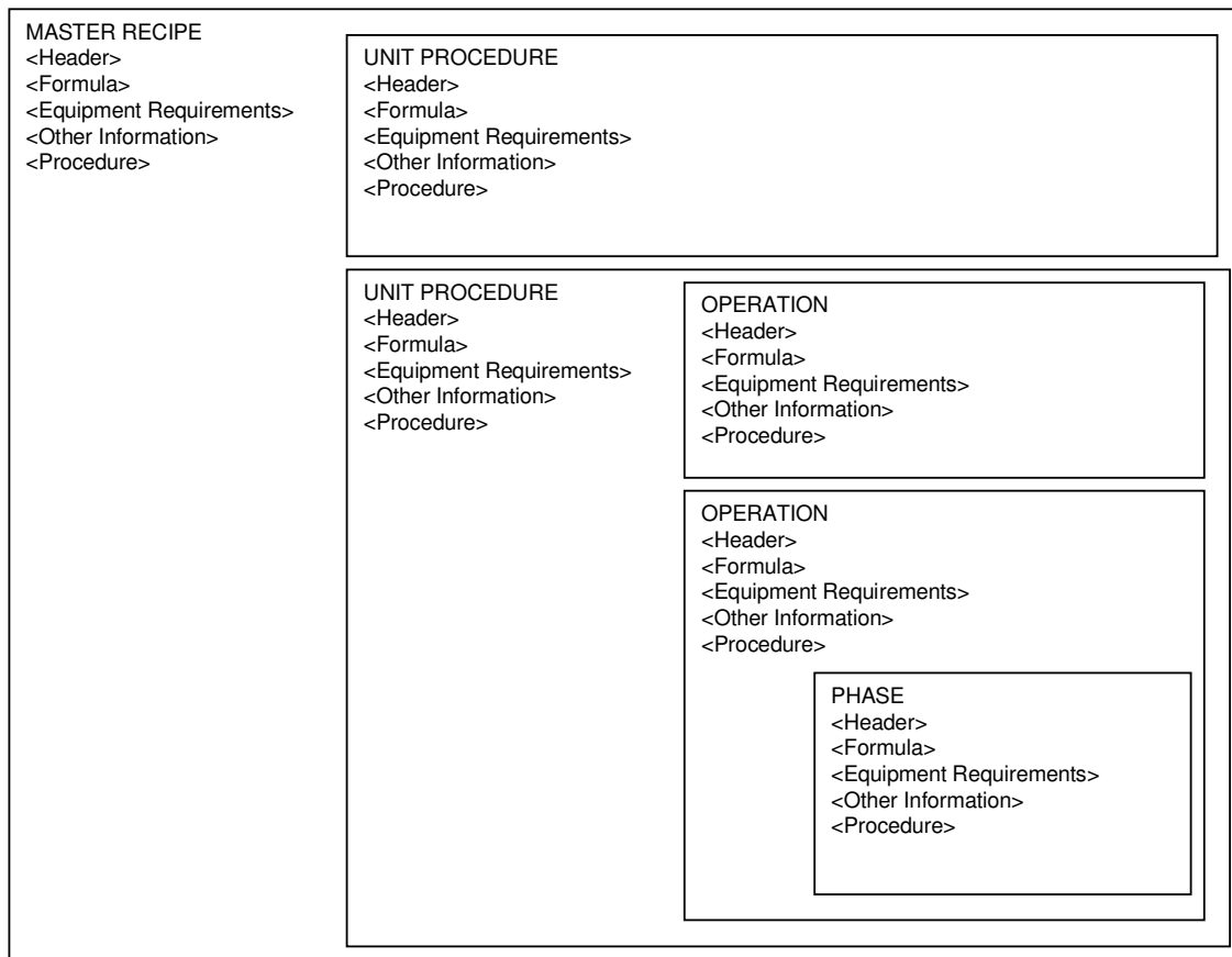
Figure 14- Recipe entity encapsulation
