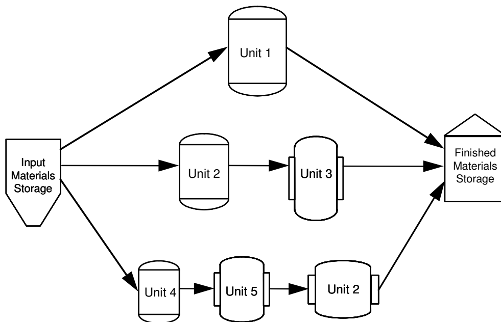
Figure 5 — Multiple-path structure
