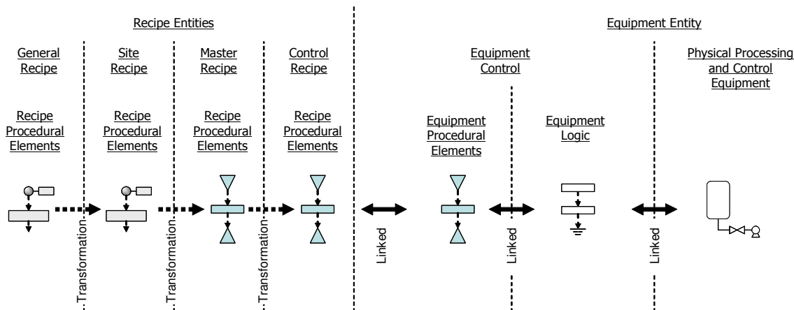
Figure 15 - Information Flow from General Recipe to Equipment Entity
