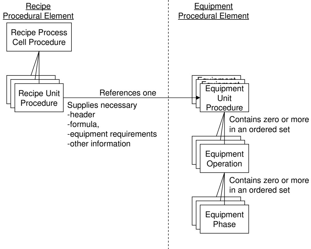
Figure 20 — Control recipe procedure example with unit procedures
