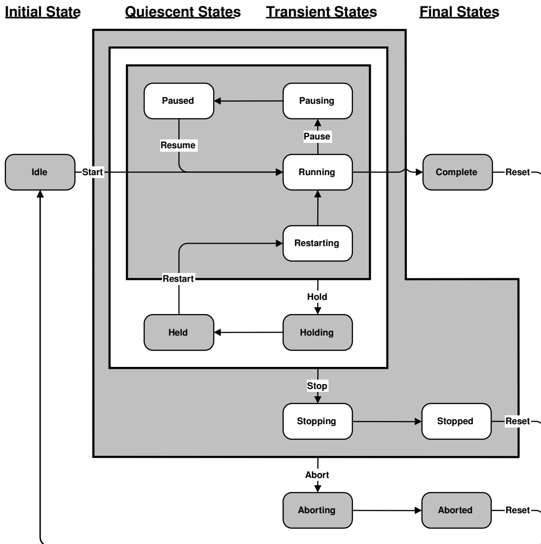
Figure 23 — State transition diagram for example states for procedural elements
