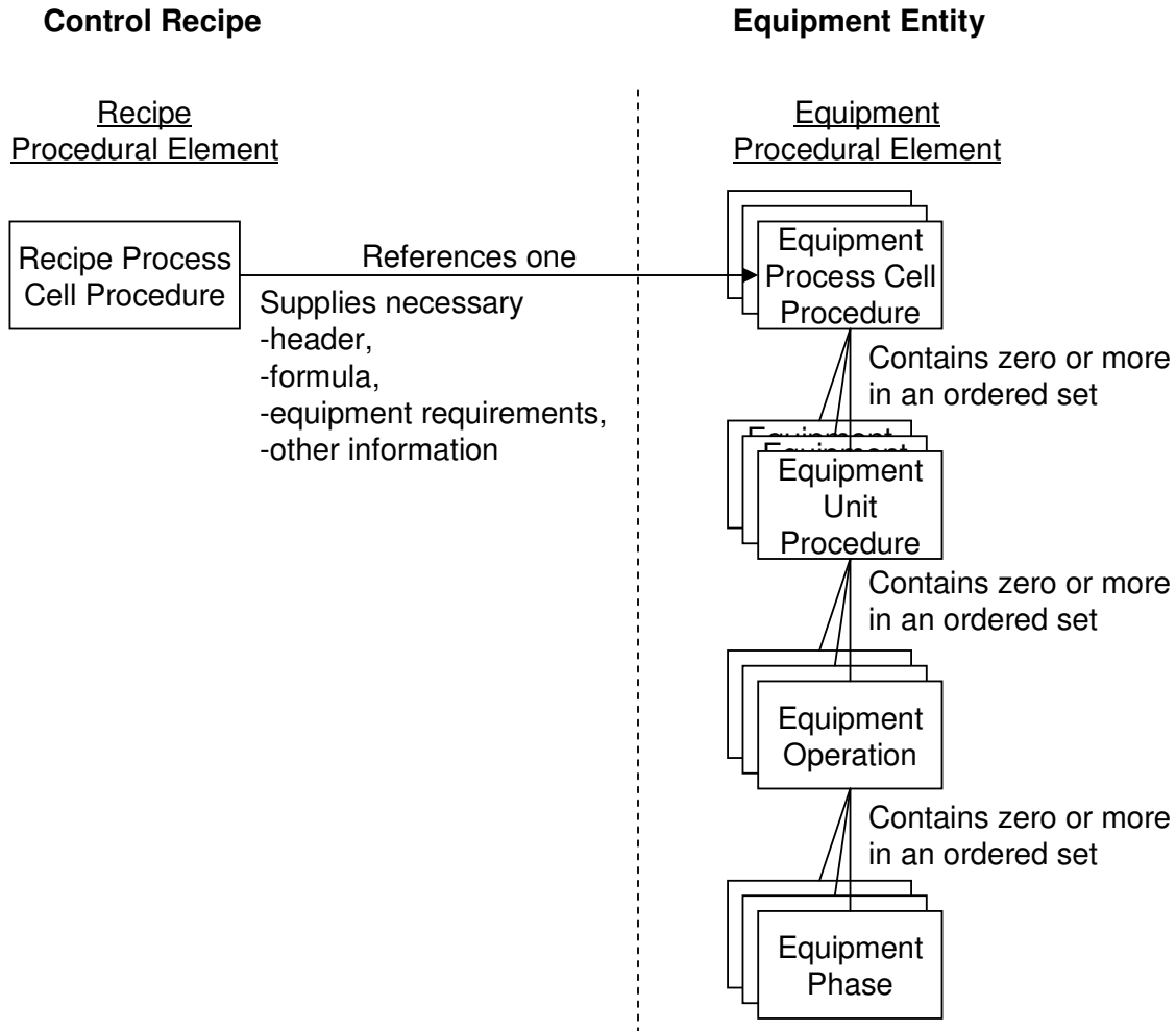
Figure 21 — Control recipe procedure example with only a process cell procedure
