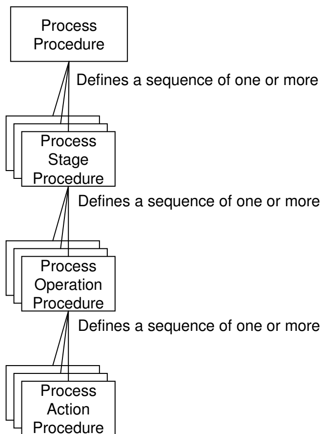
Figure 11 — General/Site recipe procedure levels
