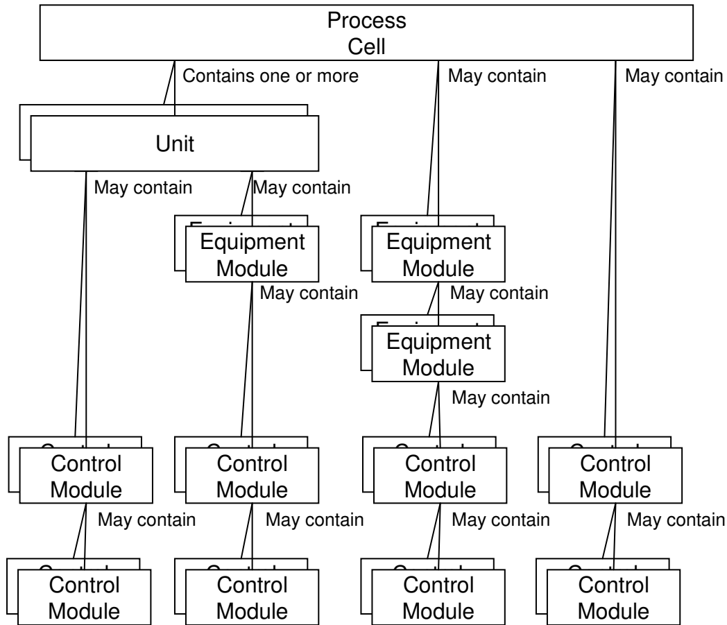
Figure 8 – Equipment Entities
