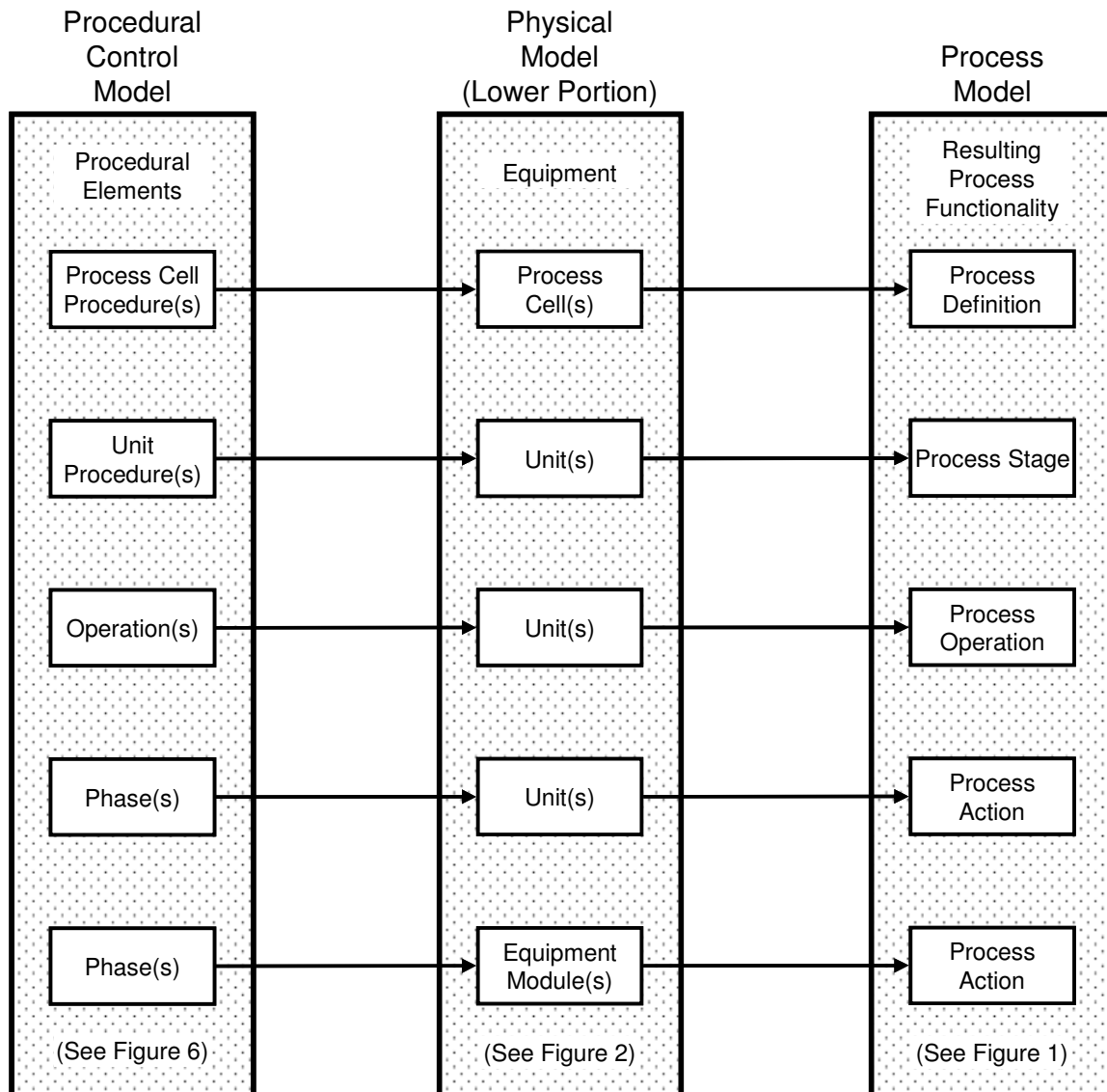
Figure 9 — Procedural control/equipment mapping to achieve process functionality
