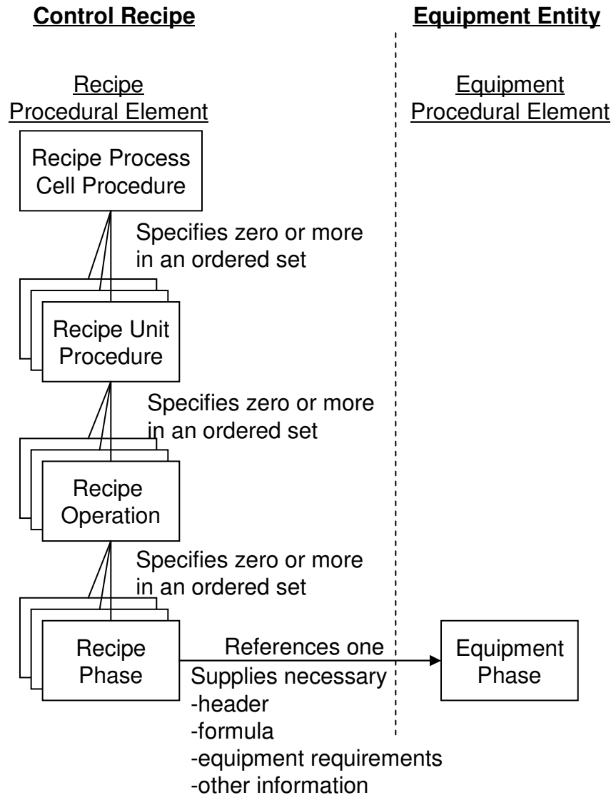
Figure 16 – Separation of the types of procedural elements and external procedural element task strategy
