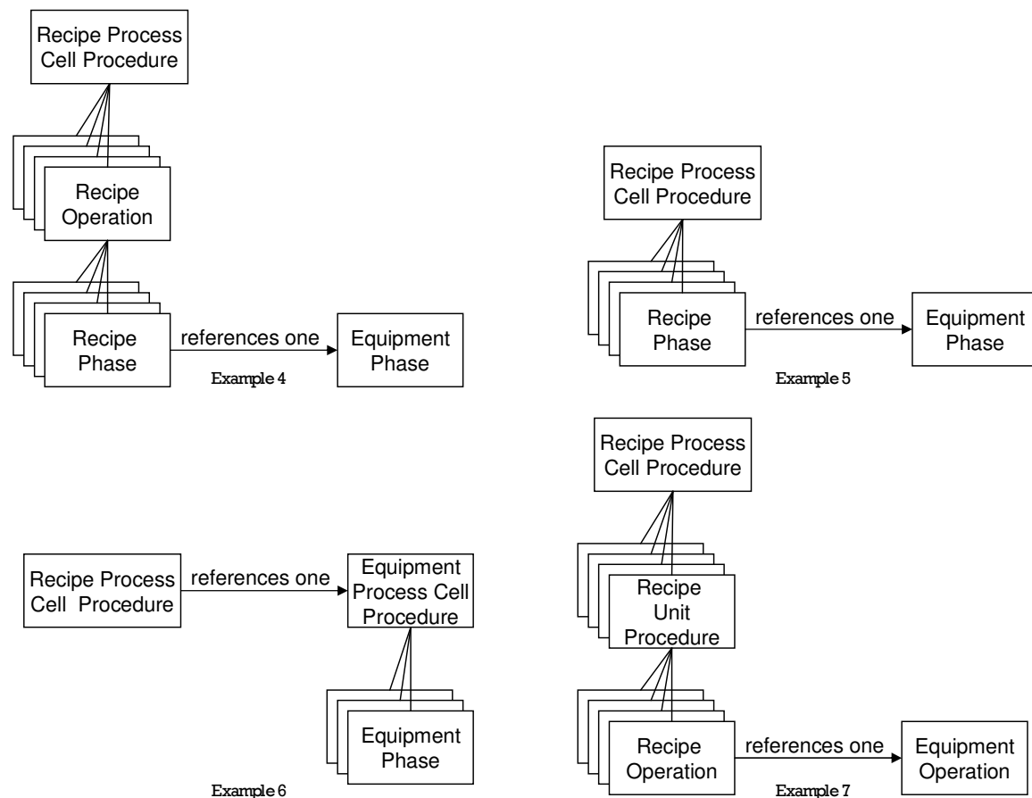
Figure 22 — Control recipe procedure/equipment control collapsibility examples
