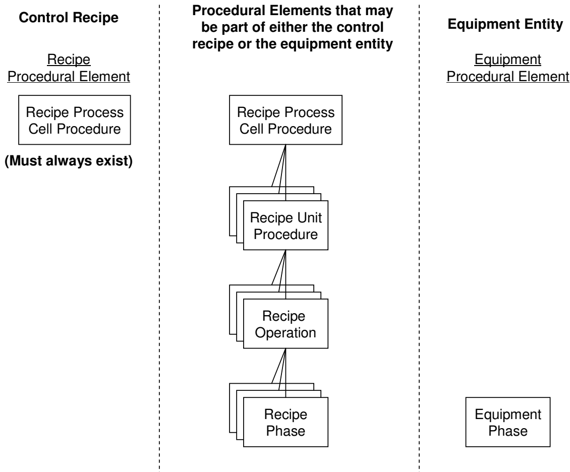
Figure 17 — Control recipe procedure/equipment control separation
